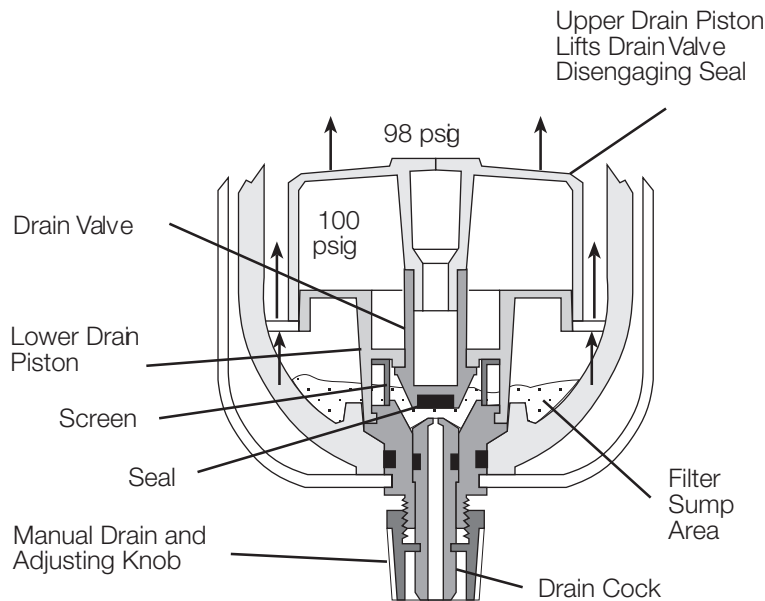
Vanguard Internal Automatic Bowl Drain
