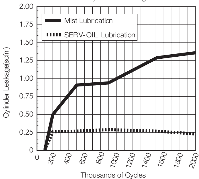
Effect of Lubrication on Cylinder Leakage
