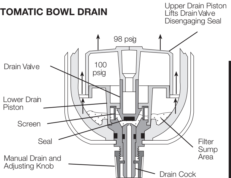
Vanguard Internal Automatic Bowl Drain
